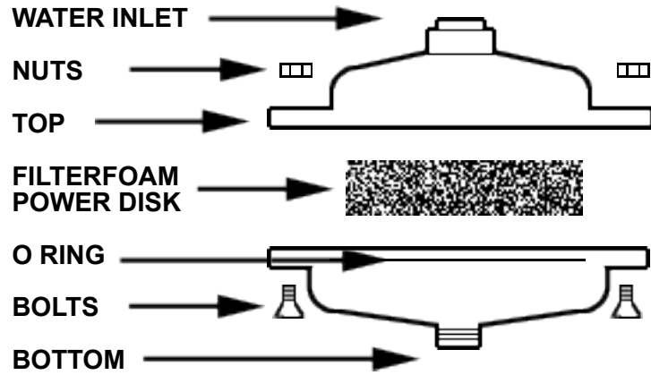
TurboShower 104 featuring the Power Disk
